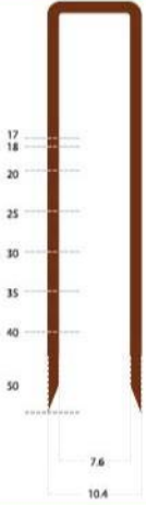
Delta Zimba Teli Delta Staple 100 serisi/series*
