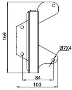
M02010255 Ürün No/Prod. No: 88 KOL BAĞLANTI MEKANİZMASI (M8 SOMUNLU) ARM CONNECTION MECHANISM (WITH M8 NUT)
