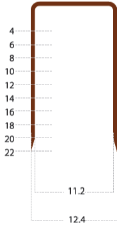
Delta Zimba Teli Delta Staple 80 serisi/series*
