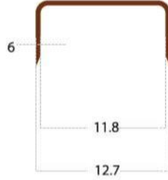
M00000206 Ürün No/Prod. No: 193 Delta Zimba Teli/Delta Staple 24/6 serisi/series*
