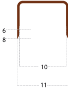
Delta Zimba Teli Delta Staple 200 serisi/series*
